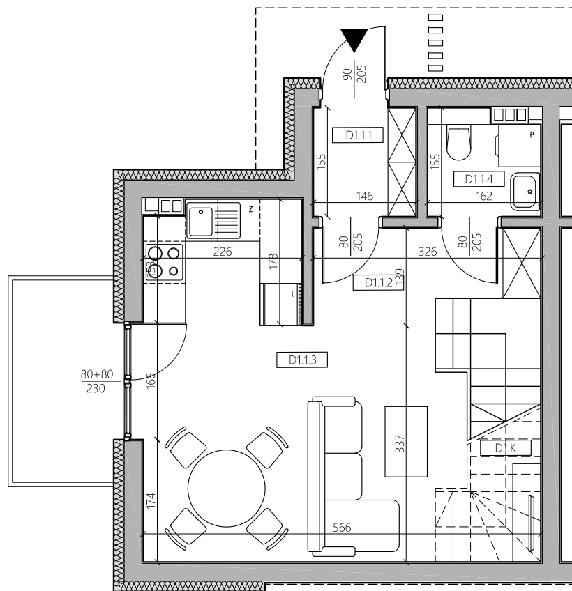
PARTER
